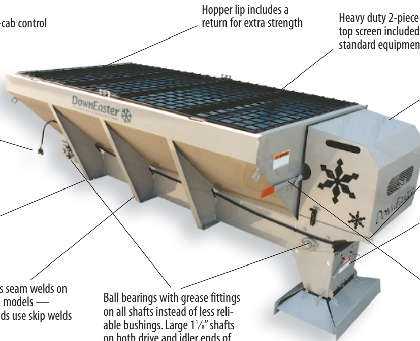
Adjustable feed gate allows you to control the flow of material — light for snow, heavy for ice or trouble spots
