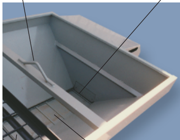
Cleaning pad minimizes material deposits in pickup bed
